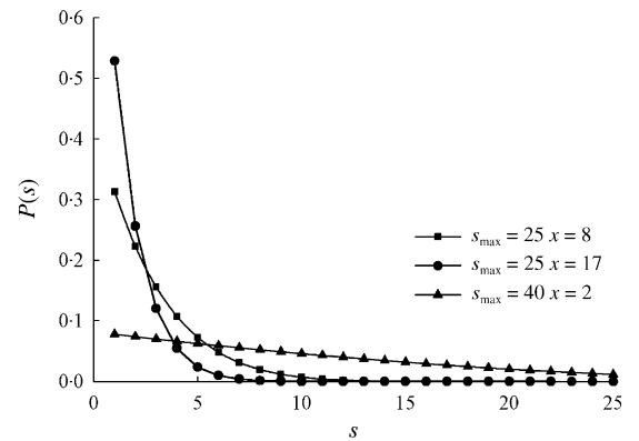
Fig. 3. Intraday step distribution for different parameter values, s_{\max} (maximum number of intraday steps) and x (exponent of equation 1, as described in the text).
